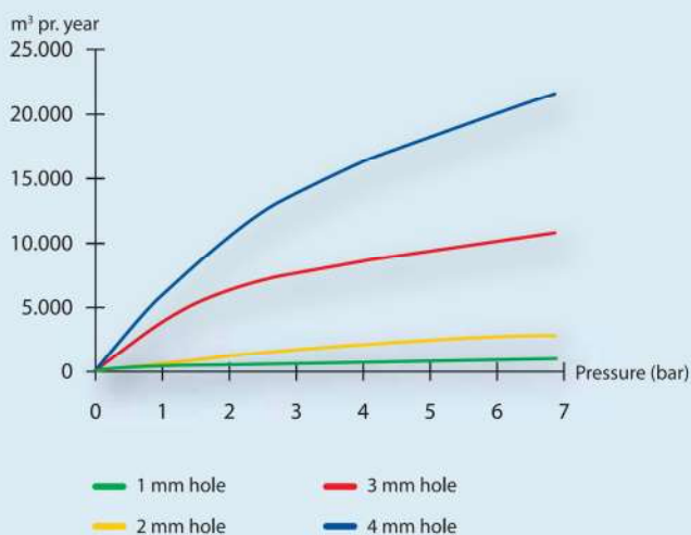
Reducing water losses by lowering system pressure becomes increasingly effective as the size of line breaks increase.
